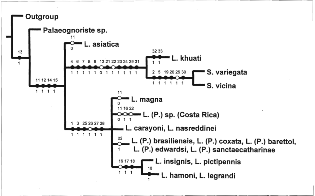
Fig. 8: Relationships of genera of Lygistorrhinidae, based on a consensus of 13 equally parsimonious trees. Length 40; CI 82; RI 87. Characters are numbered (above lines); all have a state of 1, except for those with polarity reversal (0)(below lines). Open circles are homoplasious characters.
