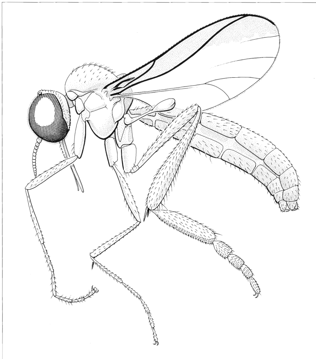
Fig. 1: Habitus of Loyugesia khuati gen. nov, spec. nov. Approximate length of fly is 2.2 mm.
