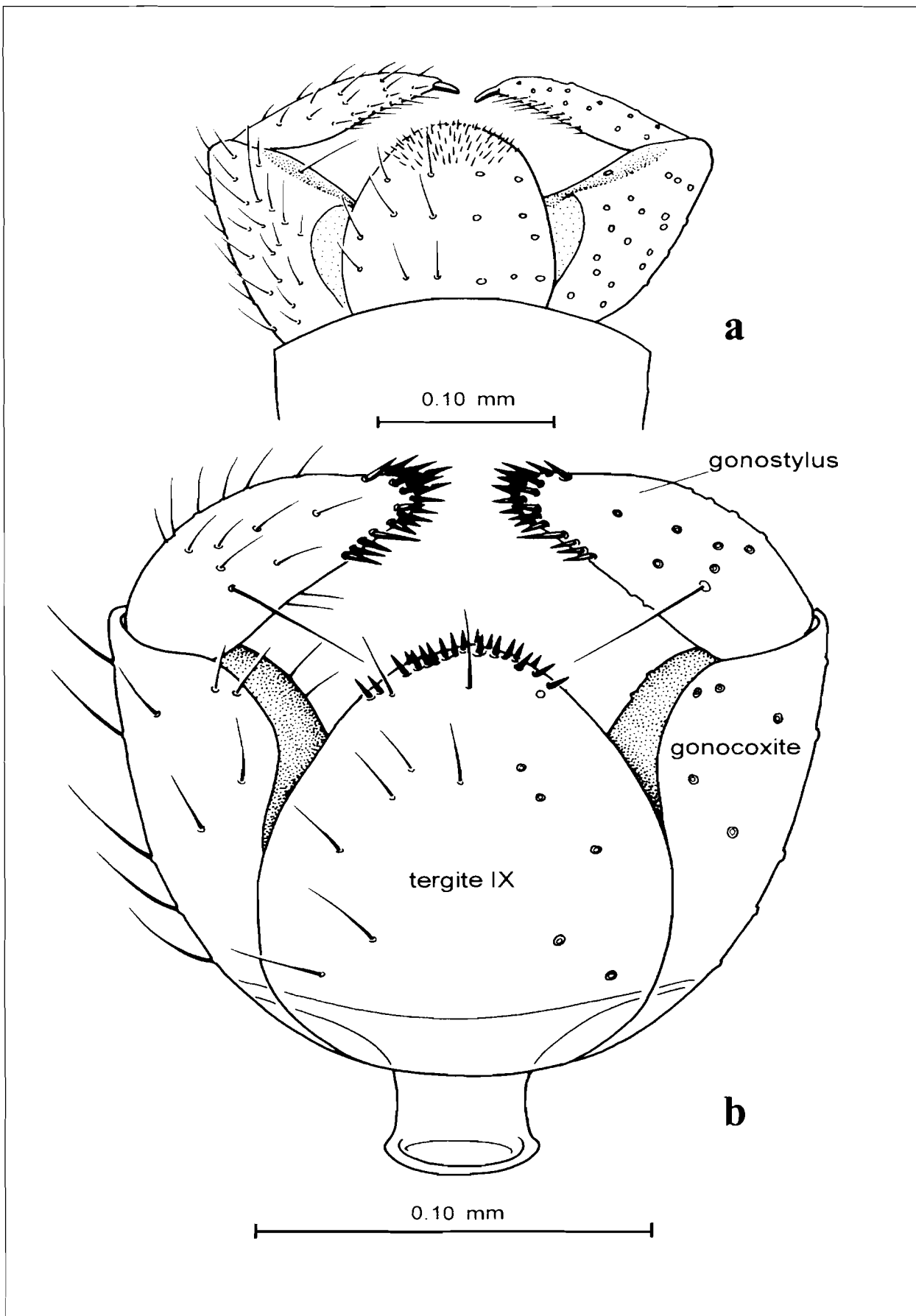
Fig. 7a, b: Male genitalia of Lygistorhinidae. – a: Palaeognoriste spec. (AMNH B-JH8); – b: Loyugesia khuati , gen. nov, spec. nov.
