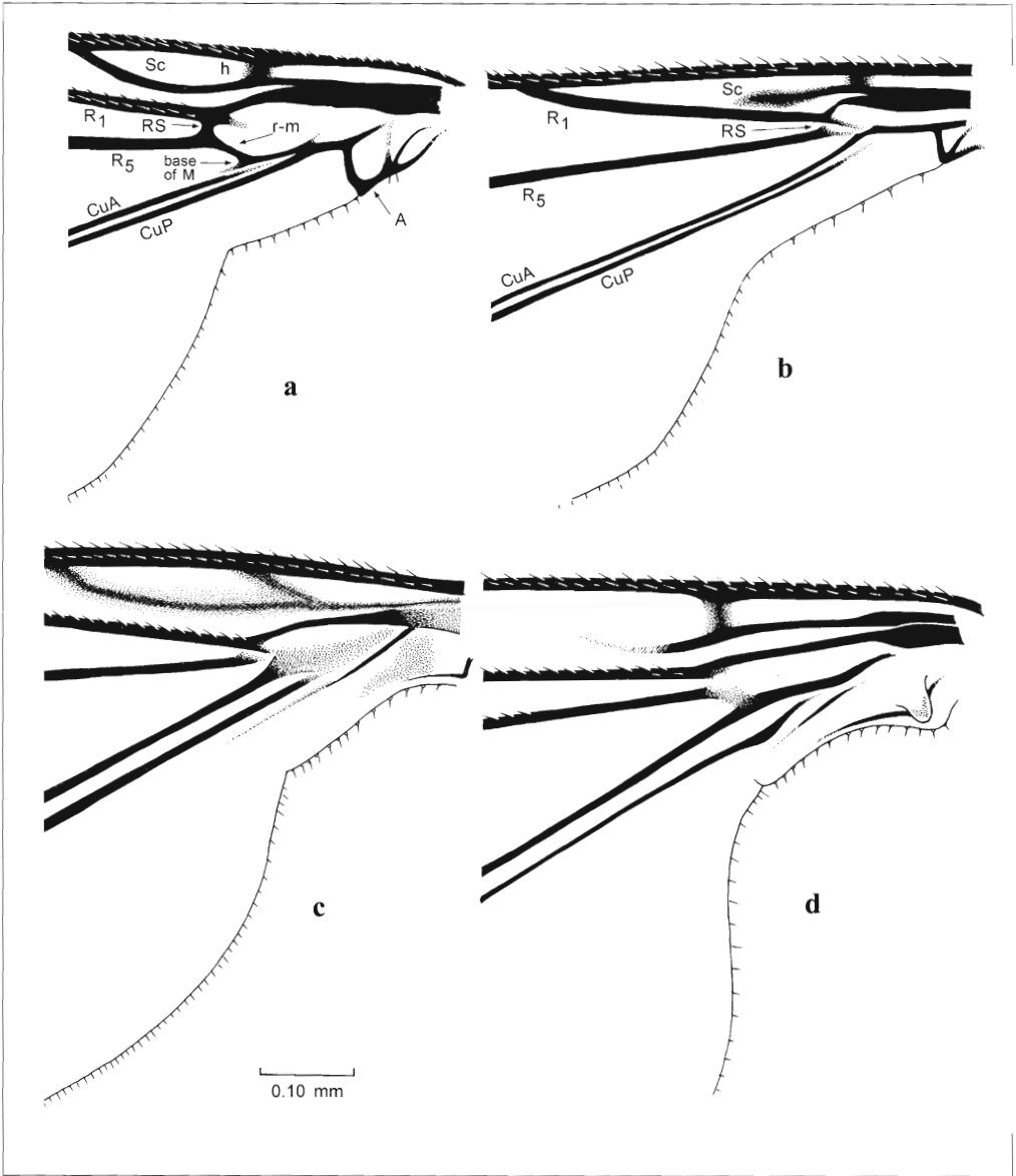
Fig. 6a-d: Bases of the wings of Lygistorrhinidae. – a: Palaeognoriste spec. (AMNH B-JH8). – b: Loyugesa khuati gen. nov, spec. nov. – c: “ Lygistorrhina ” asiatica SENIOR-WHITE. – d: Lygistorrhina sanctaecatherinae THOMPSON.
